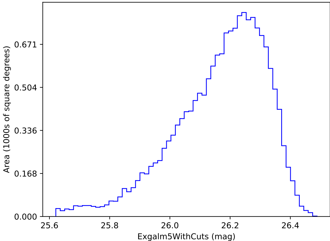
noroll_mjdp270_v3.4_10yrs i band non-DD year 6: ExgalM5WithCuts
