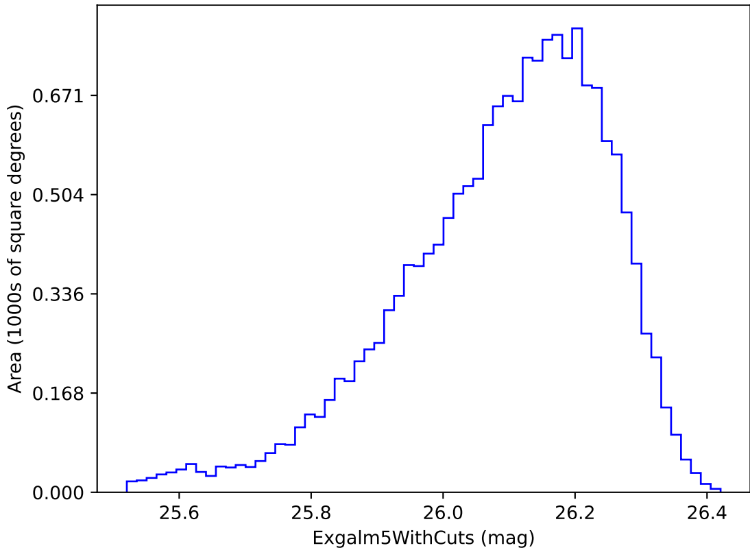
noroll_mjdp270_v3.4_10yrs i band non-DD year 5: ExgalM5WithCuts
