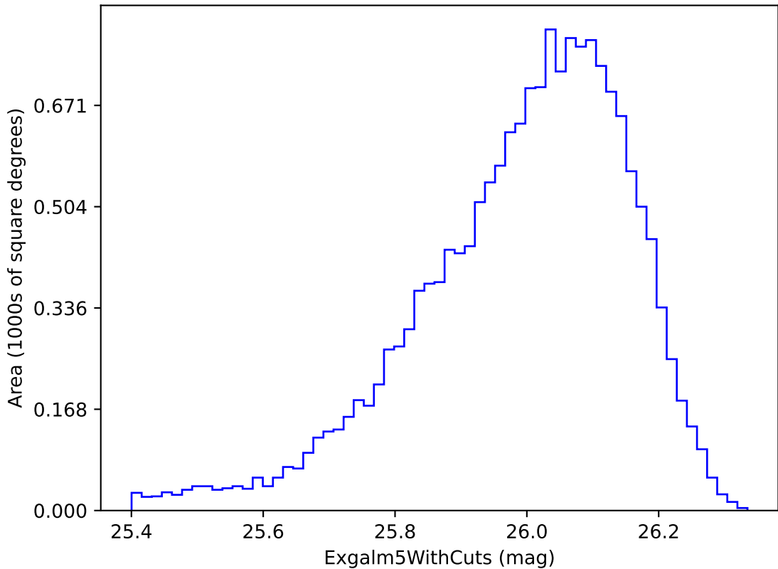
noroll_mjdp270_v3.4_10yrs i band non-DD year 4: ExgalM5WithCuts
