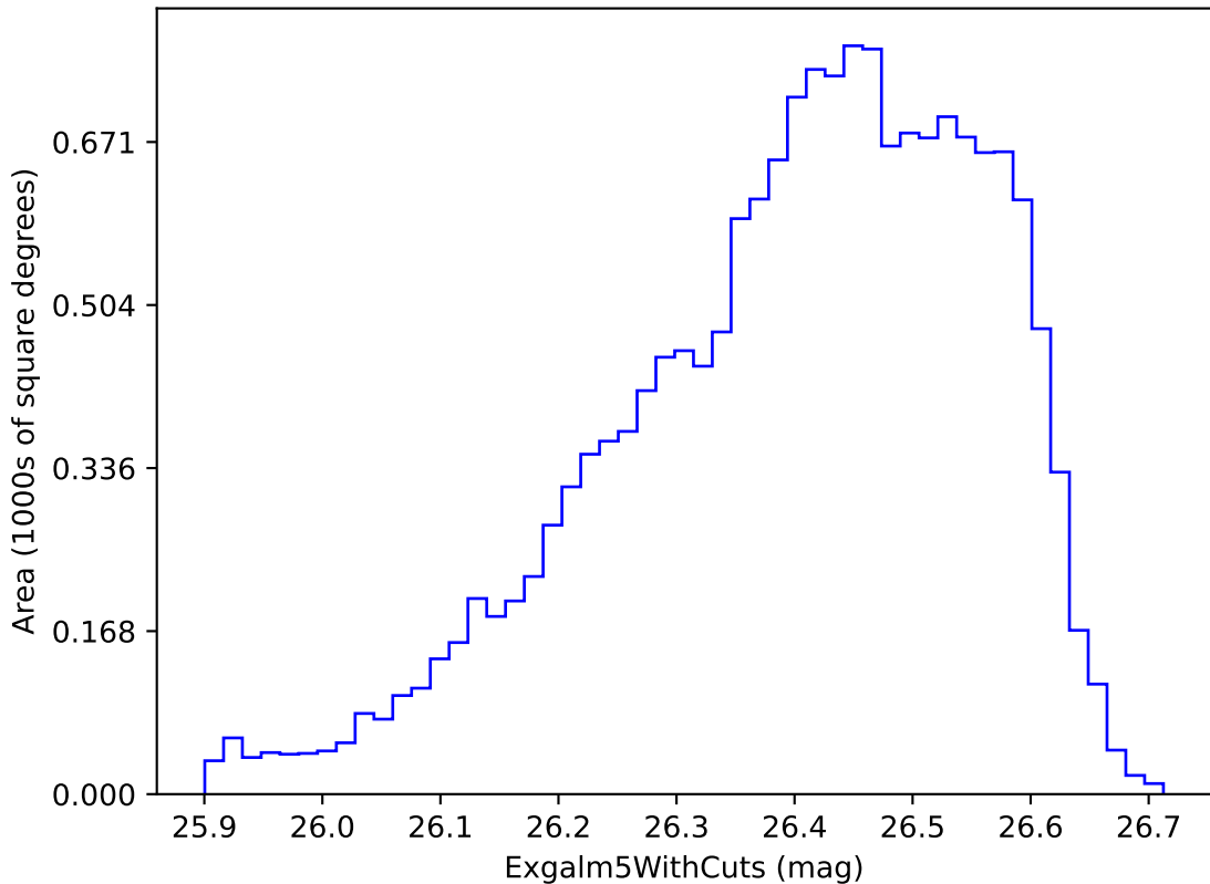
noroll_mjdp270_v3.4_10yrs i band non-DD year 10: Exgal5WithCuts
