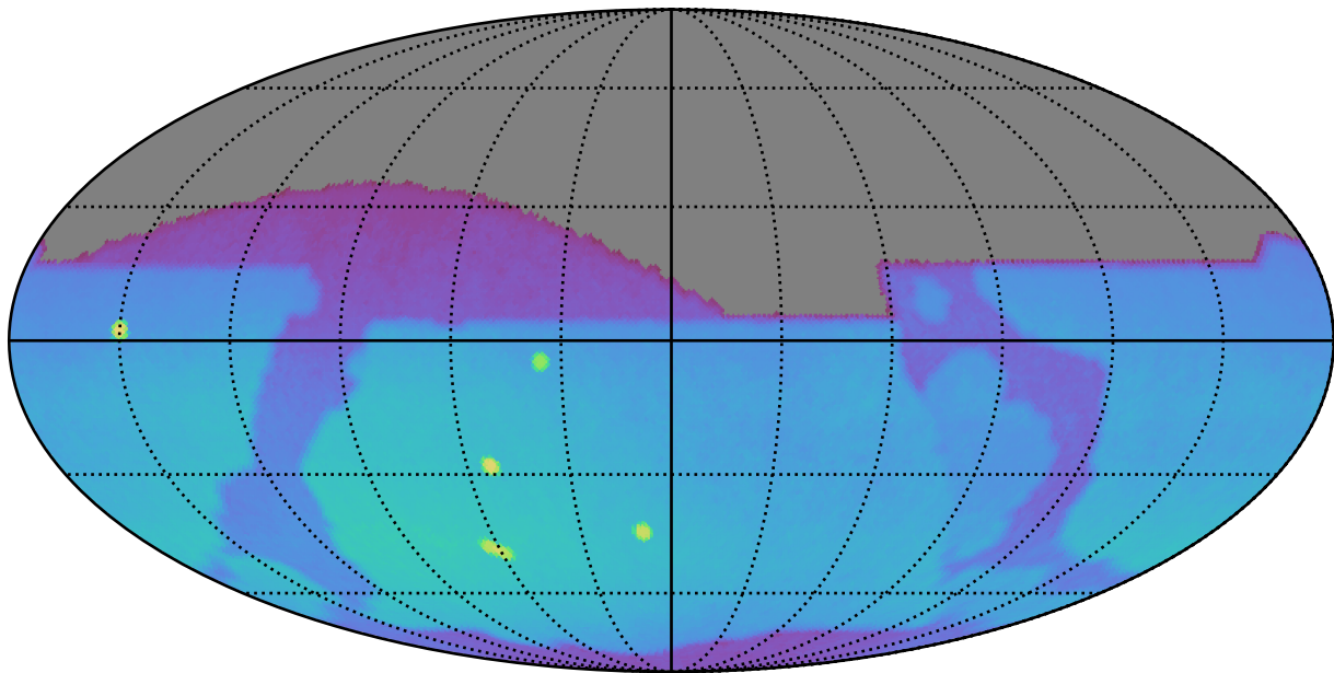
noroll_mjdp270_v3.4_10yrs : Brown Dwarf, L7
