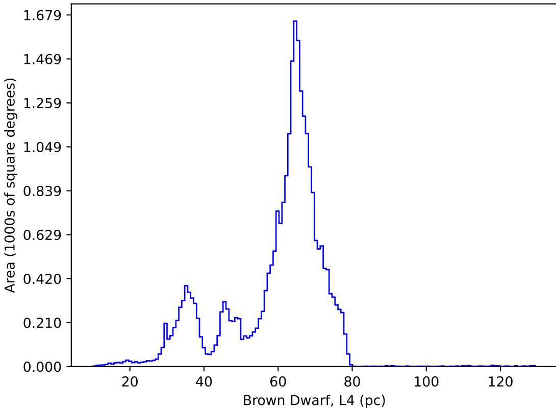
noroll_mjdp270_v3.4_10yrs : Brown Dwarf, L4
