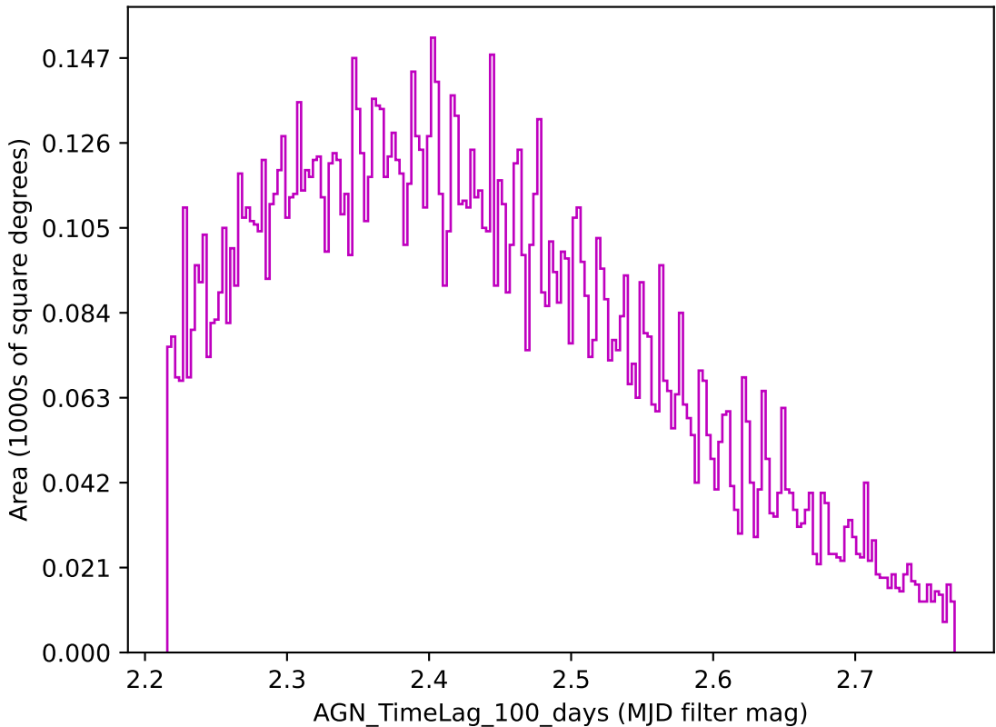
noroll_mjdp270_v3.4_10yrs z band: AGN_TimeLag_100_days
