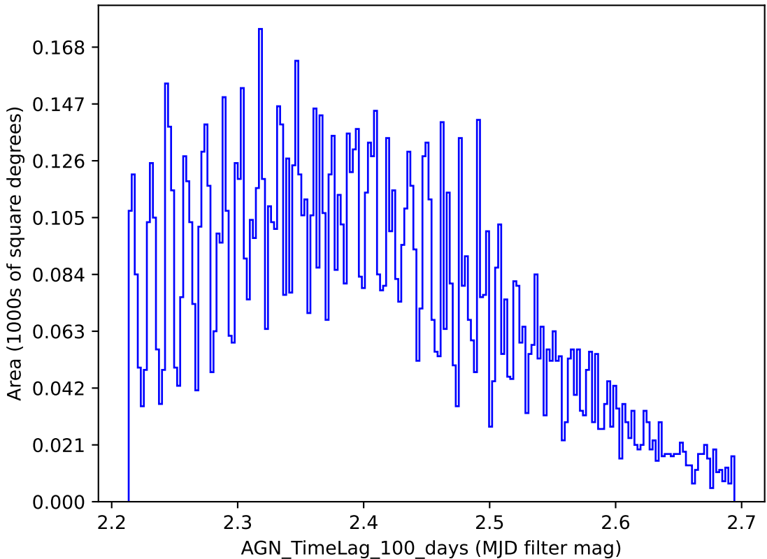
noroll_mjdp270_v3.4_10yrs y band: AGN_TimeLag_100_days
