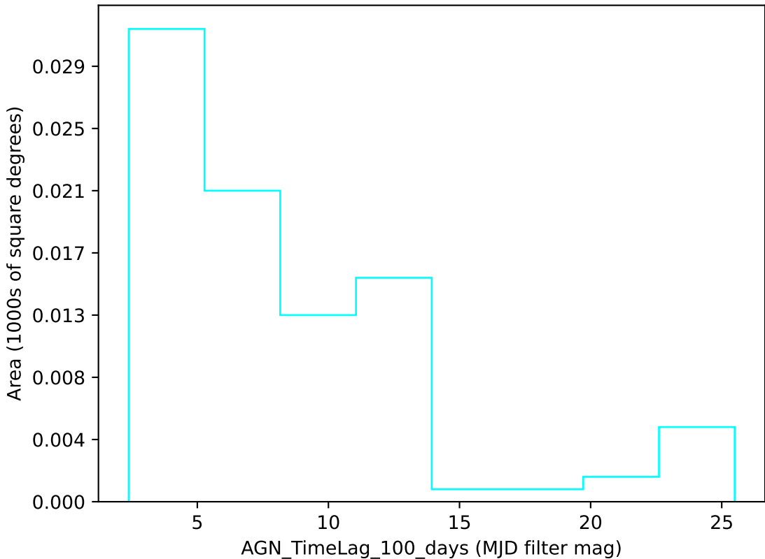
noroll_mjdp270_v3.4_10yrs u band: AGN_TimeLag_100_days
