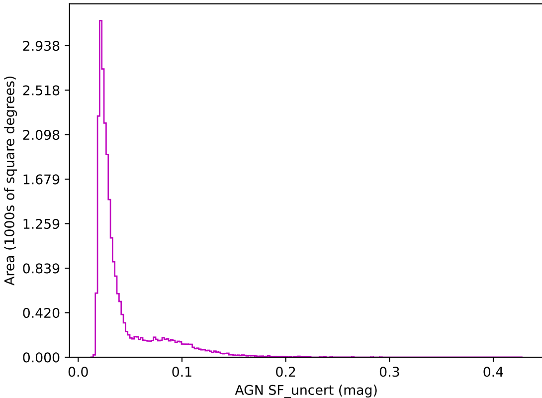
noroll_mjdp270_v3.4_10yrs z band: AGN SF_uncert
