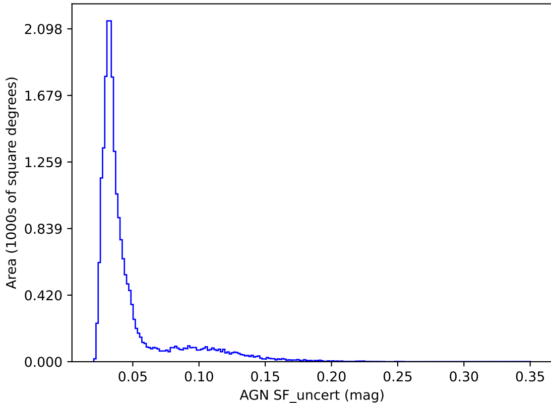
noroll_mjdp270_v3.4_10yrs y band: AGN SF_uncert
