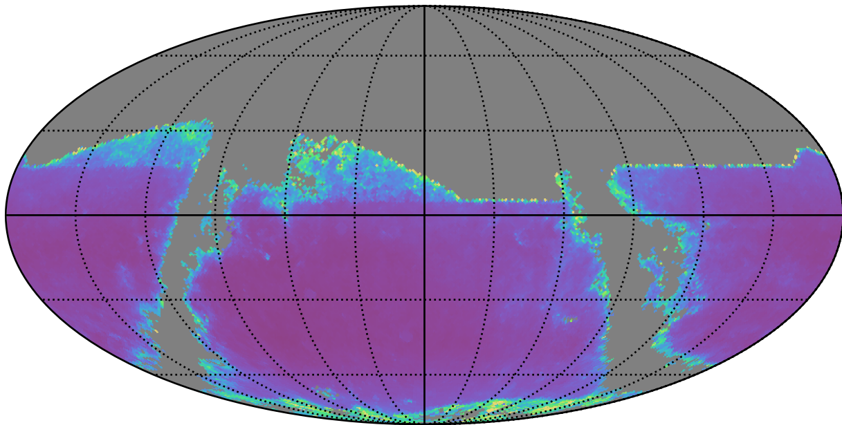
noroll_mjdp270_v3.4_10yrs r band: AGN SF_uncert
