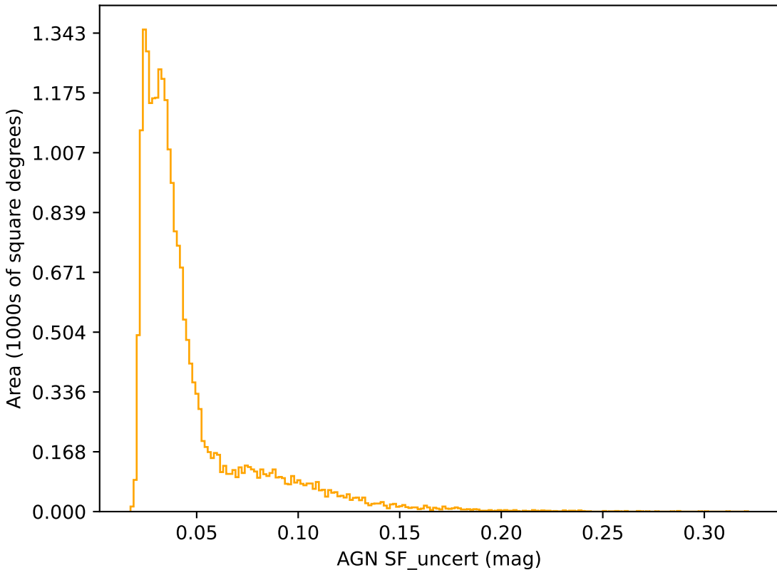
noroll_mjdp270_v3.4_10yrs r band: AGN SF_uncert
