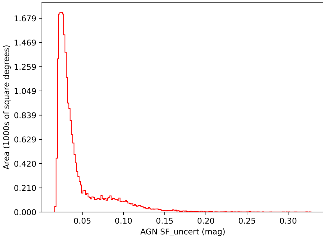
noroll_mjdp270_v3.4_10yrs i band: AGN SF_uncert
