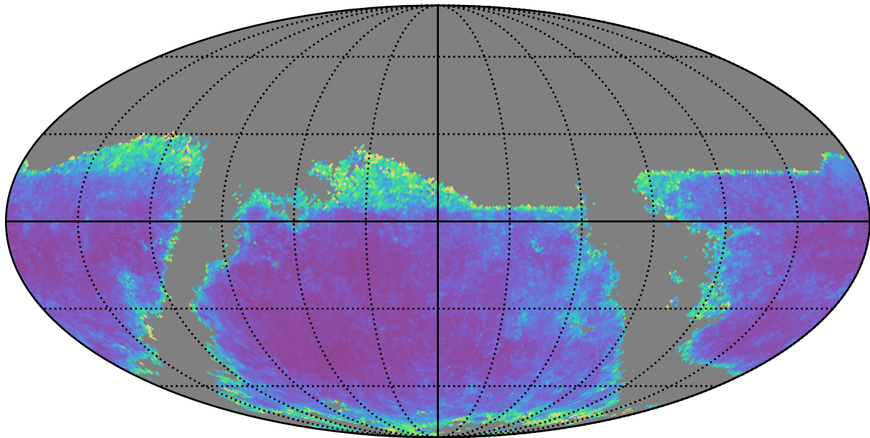
noroll_mjdp270_v3.4_10yrs g band: AGN SF_uncert
