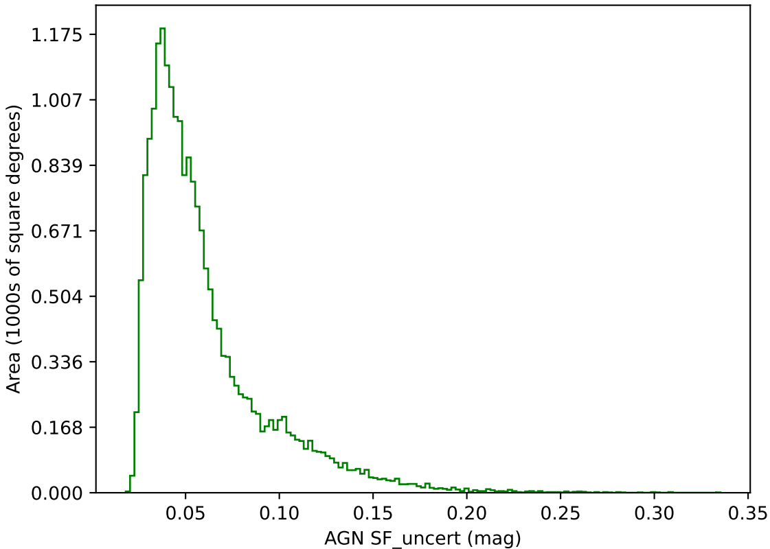
noroll_mjdp270_v3.4_10yrs g band: AGN SF_uncert
