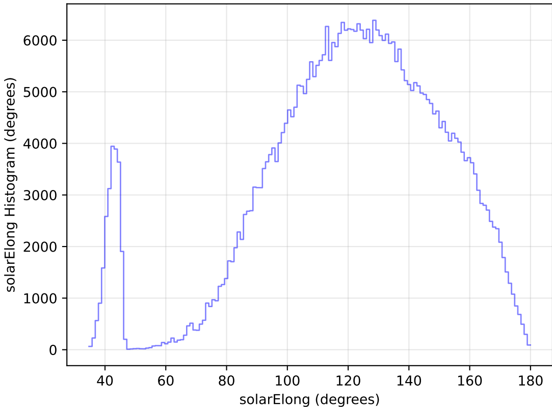
noroll_mjdp270_v3.4_10yrs WFD z band: solarElong Histogram
