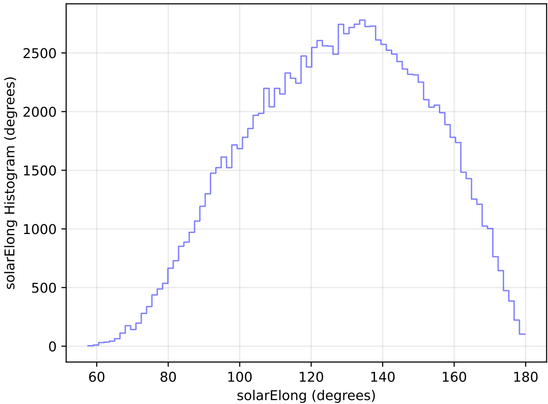
noroll_mjdp270_v3.4_10yrs WFD u band: solarElong Histogram
