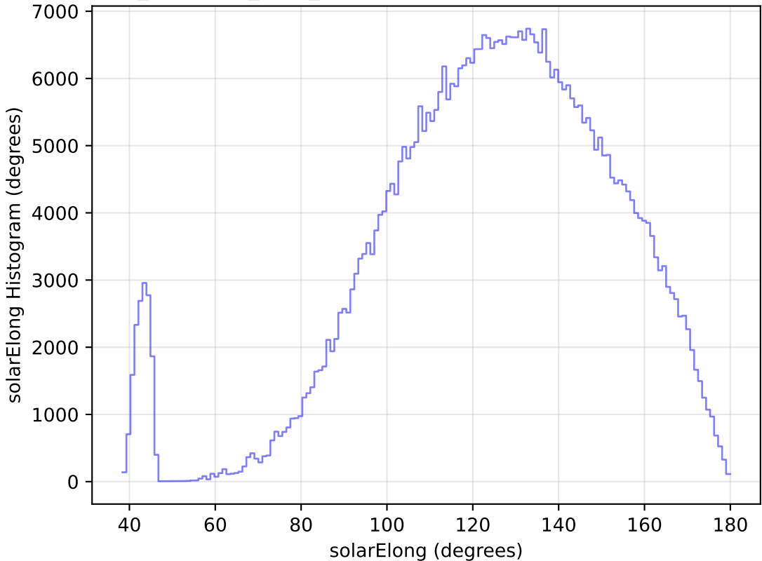
noroll_mjdp270_v3.4_10yrs WFD r band: solarElong Histogram
