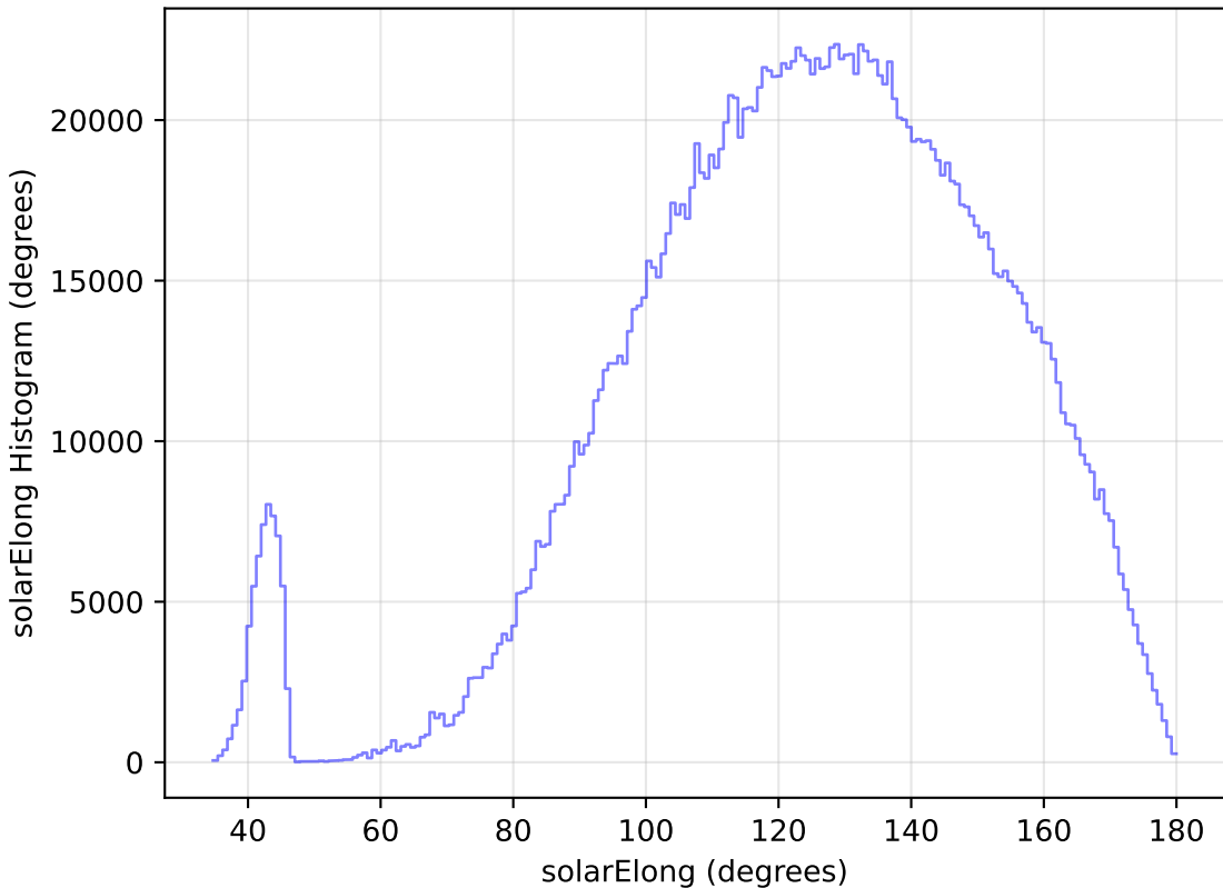
noroll_mjdp270_v3.4_10yrs WFD all bands: solarElong Histogram
