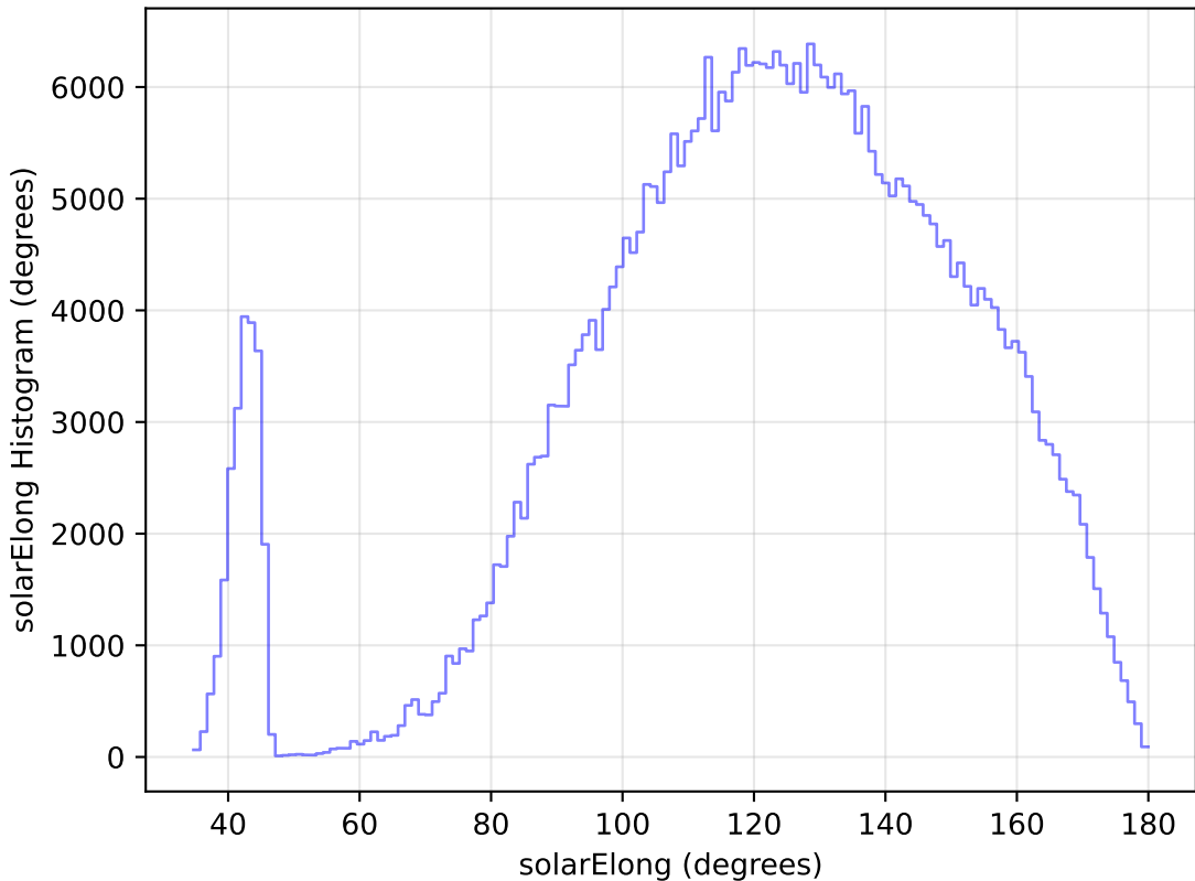
noroll_mjdp270_v3.4_10yrs All sky z band: solarElong Histogram
