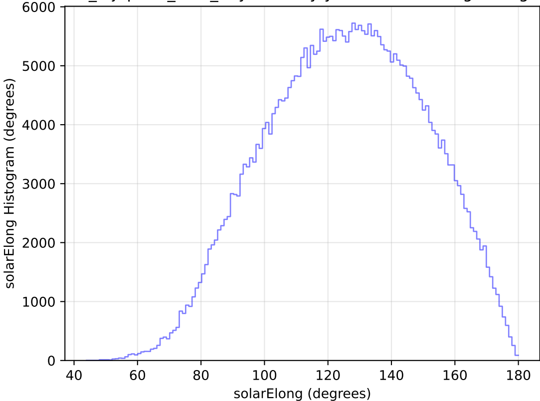
noroll_mjdp270_v3.4_10yrs All sky y band: solarElong Histogram
