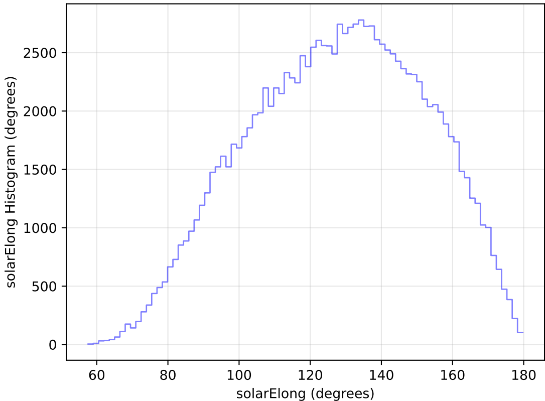
noroll_mjdp270_v3.4_10yrs All sky u band: solarElong Histogram
