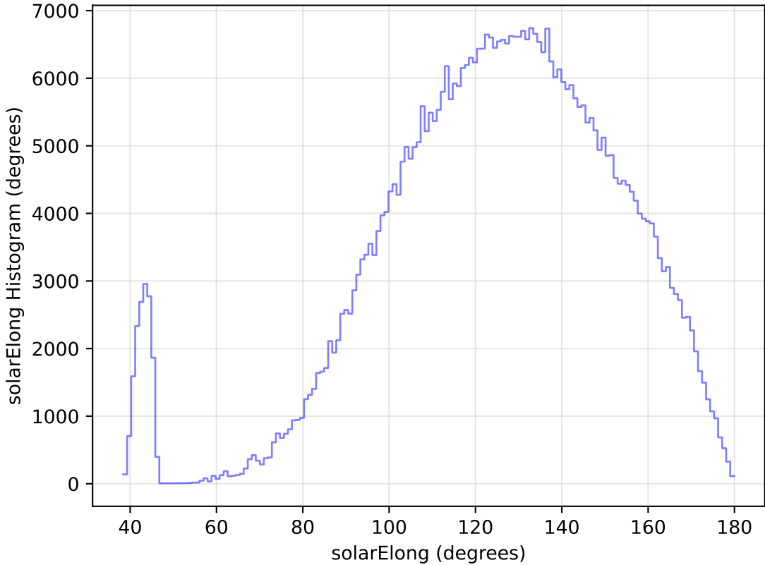
noroll_mjdp270_v3.4_10yrs All sky r band: solarElong Histogram
