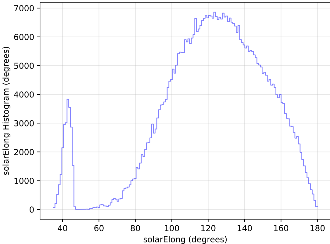
noroll_mjdp270_v3.4_10yrs All sky i band: solarElong Histogram
