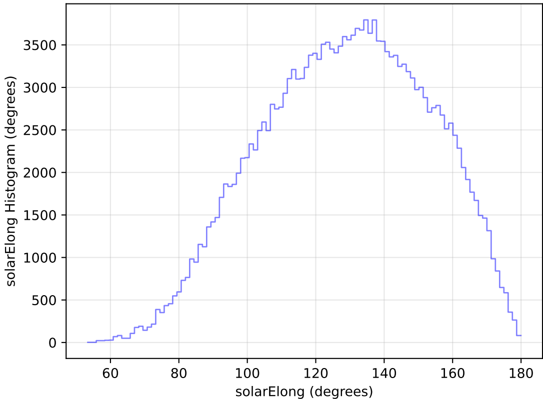
noroll_mjdp270_v3.4_10yrs All sky g band: solarElong Histogram
