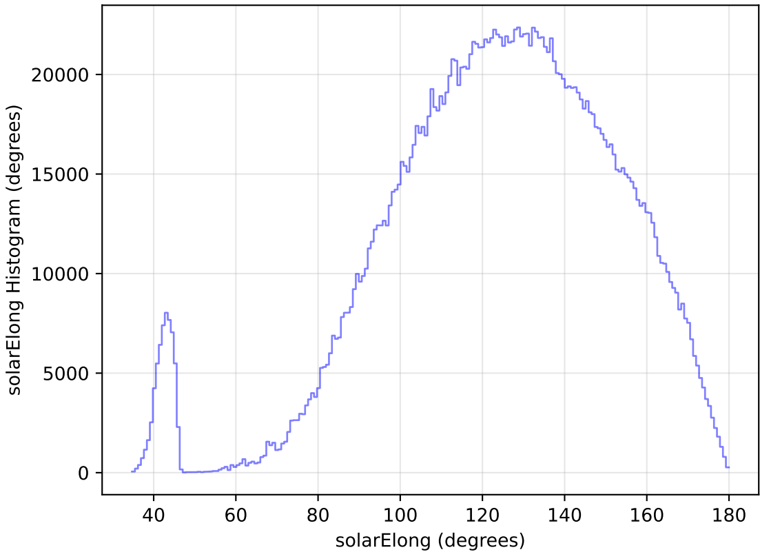
noroll_mjdp270_v3.4_10yrs All sky all bands: solarElong Histogram
