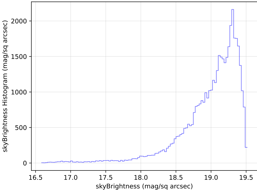
noroll_mjdp270_v3.4_10yrs Yr 1 z band: skyBrightness Histogram
