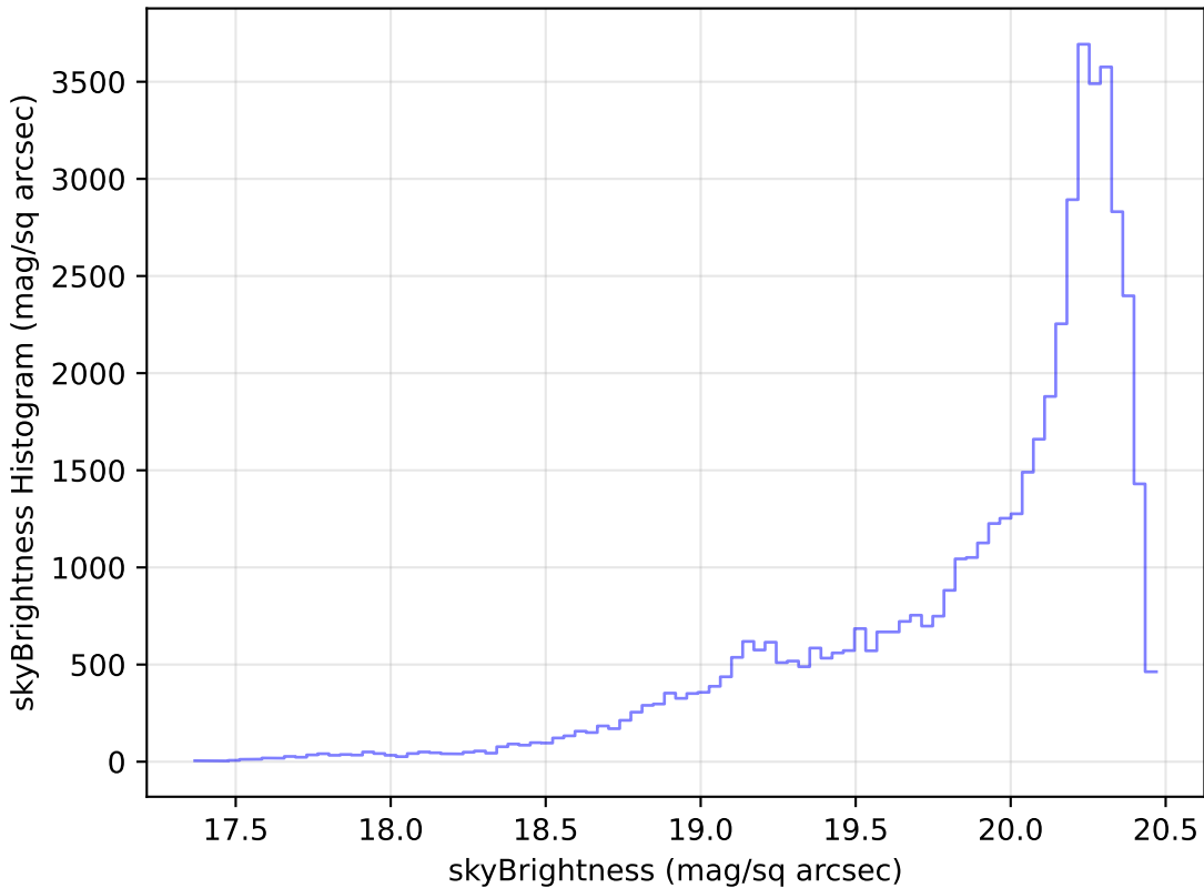
noroll_mjdp270_v3.4_10yrs Yr 1 i band: skyBrightness Histogram
