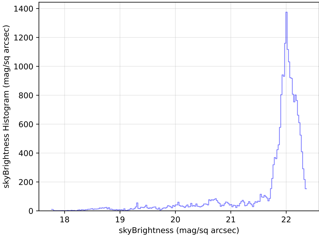
noroll_mjdp270_v3.4_10yrs Yr 1 g band: skyBrightness Histogram
