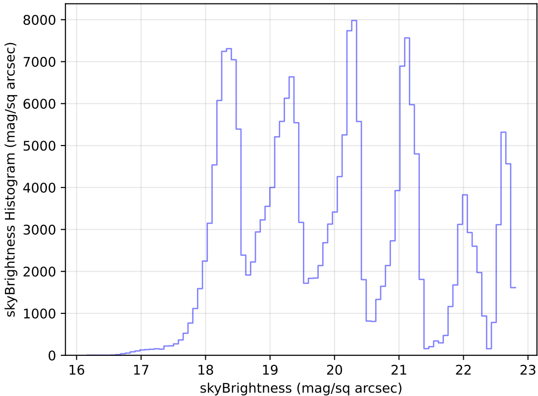
noroll_mjdp270_v3.4_10yrs Yr 1 all bands: skyBrightness Histogram
