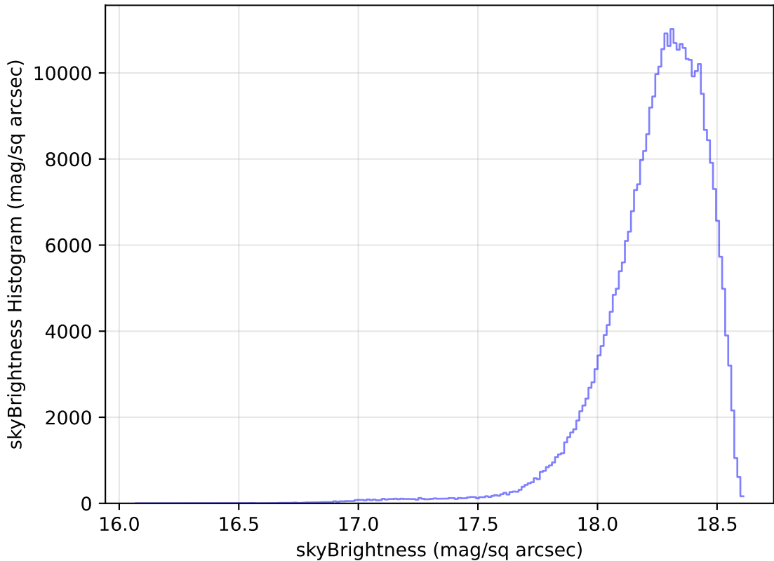
noroll_mjdp270_v3.4_10yrs WFD y band: skyBrightness Histogram
