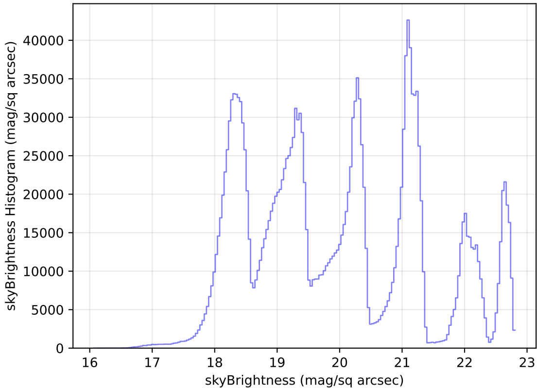
noroll_mjdp270_v3.4_10yrs WFD all bands: skyBrightness Histogram
