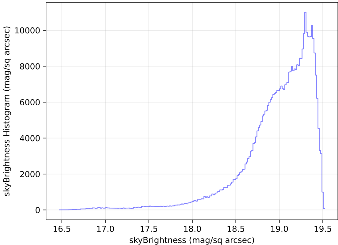
noroll_mjdp270_v3.4_10yrs All sky z band: skyBrightness Histogram
