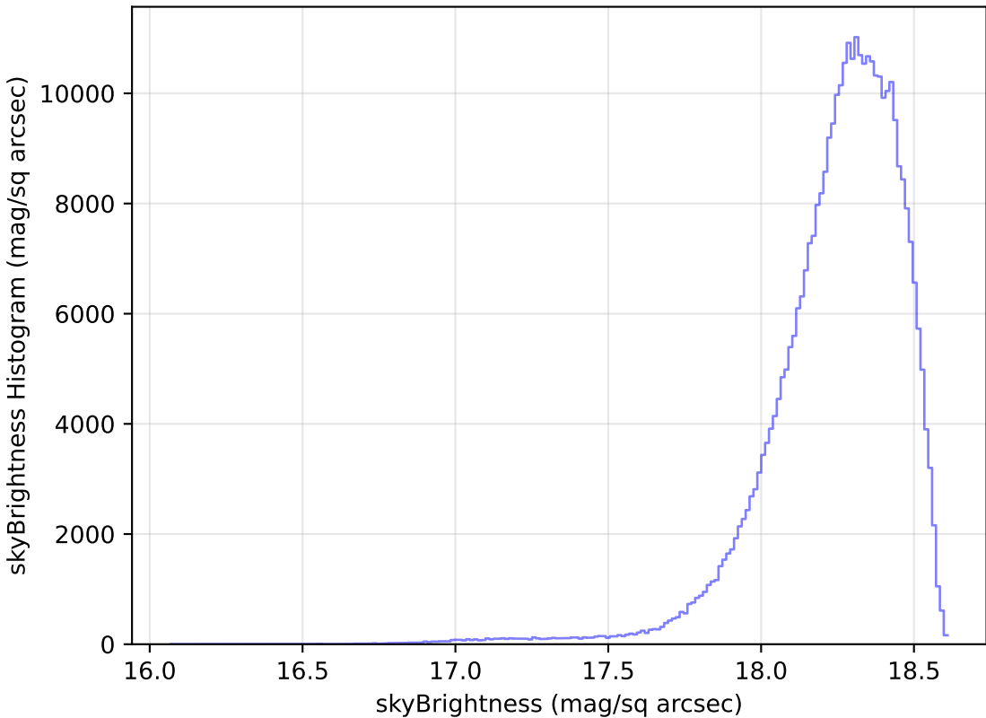
noroll_mjdp270_v3.4_10yrs All sky y band: skyBrightness Histogram
