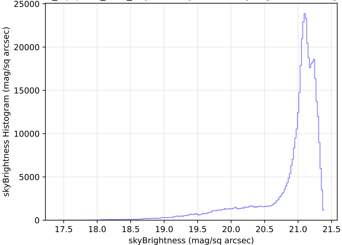
noroll_mjdp270_v3.4_10yrs All sky r band: skyBrightness Histogram
