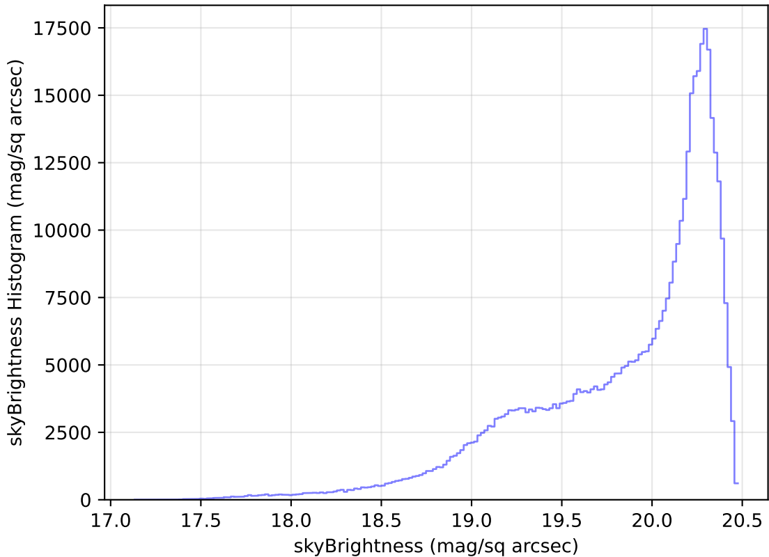
noroll_mjdp270_v3.4_10yrs All sky i band: skyBrightness Histogram
