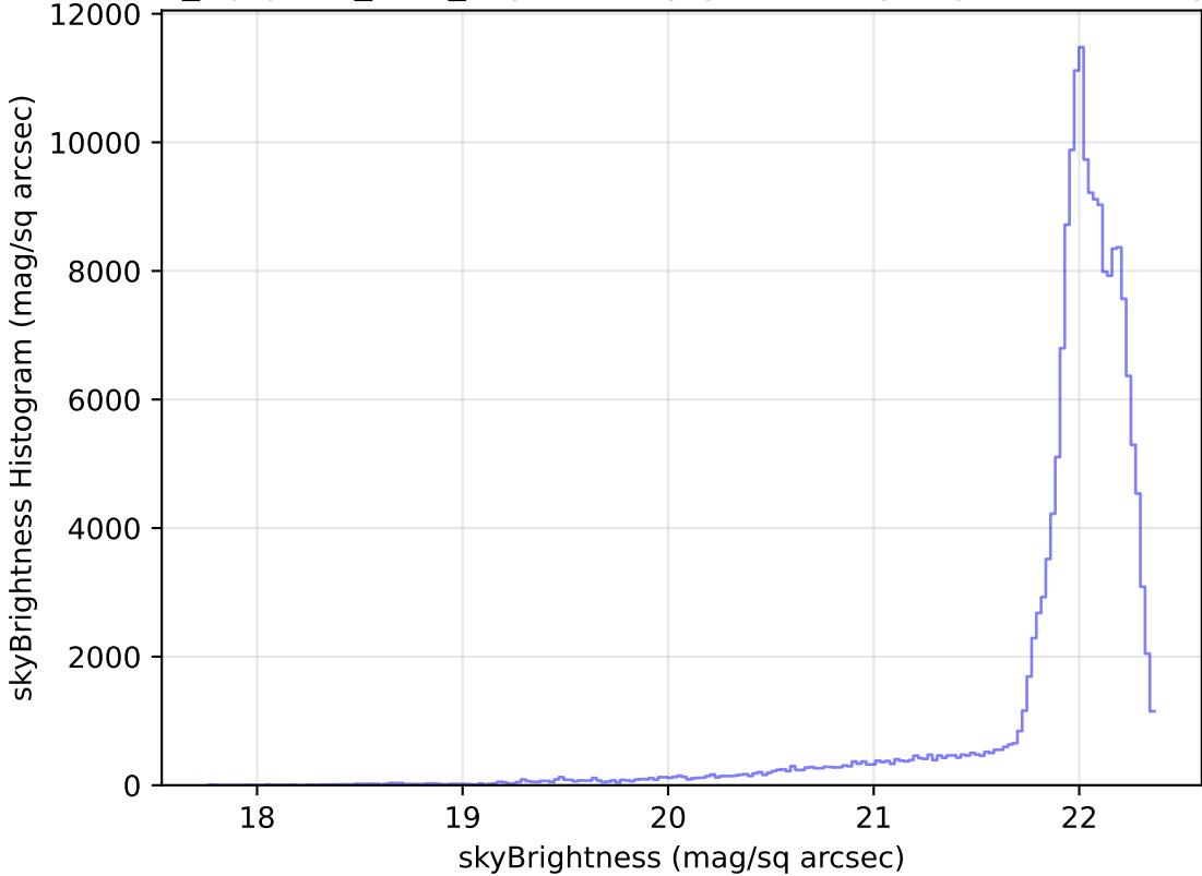
noroll_mjdp270_v3.4_10yrs All sky g band: skyBrightness Histogram
