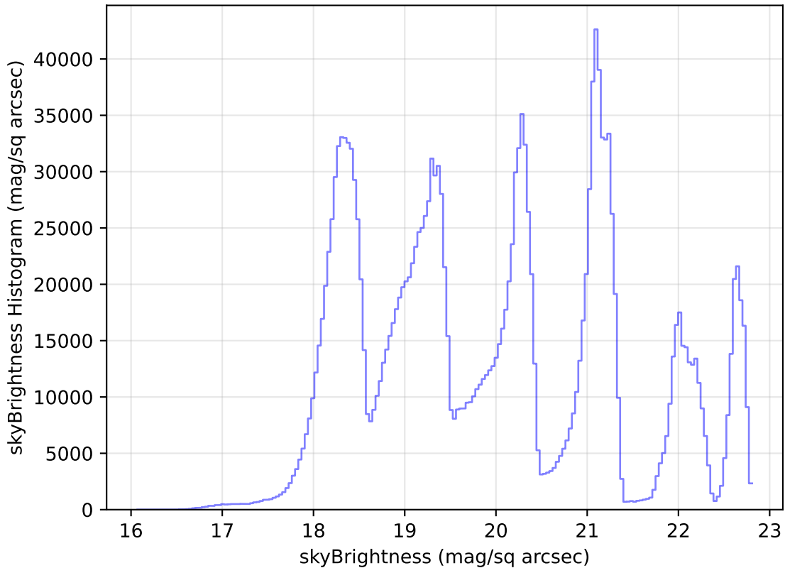
noroll_mjdp270_v3.4_10yrs All sky all bands: skyBrightness Histogram
