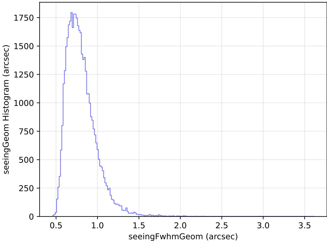
noroll_mjdp270_v3.4_10yrs Yr 1 y band: seeingGeom Histogram
