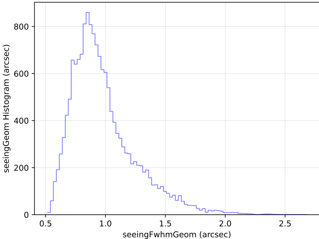
noroll_mjdp270_v3.4_10yrs Yr 1 u band: seeingGeom Histogram
