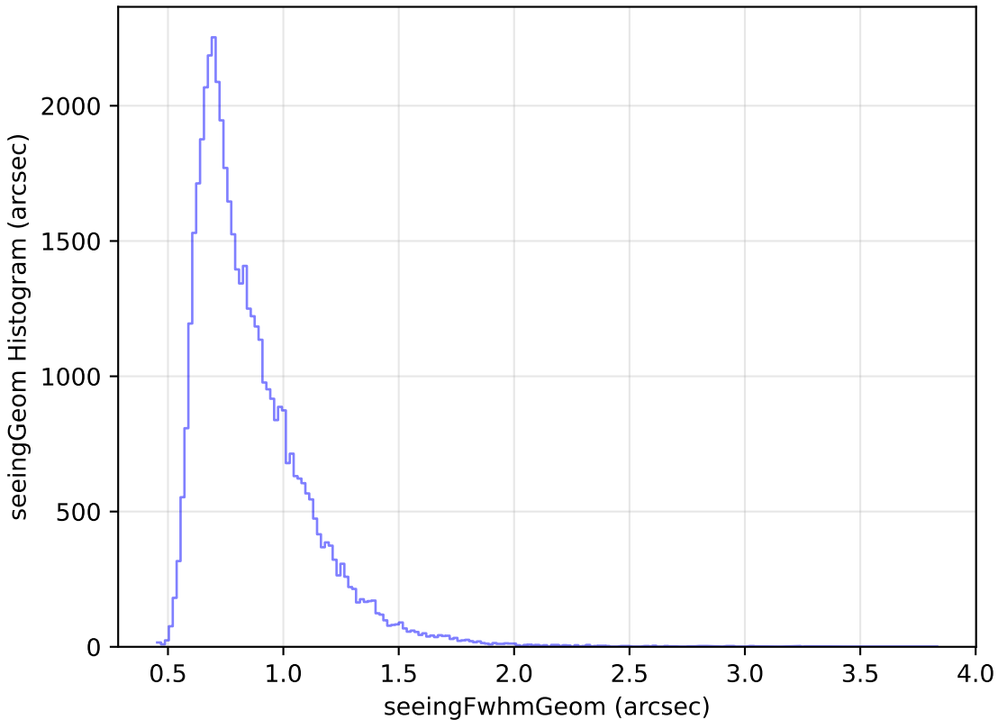
noroll_mjdp270_v3.4_10yrs Yr 1 r band: seeingGeom Histogram
