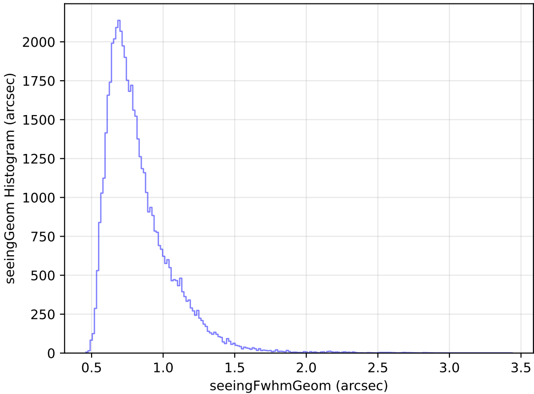
noroll_mjdp270_v3.4_10yrs Yr 1 i band: seeingGeom Histogram
