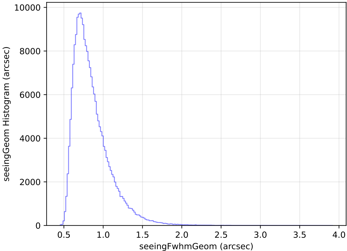
noroll_mjdp270_v3.4_10yrs Yr 1 all bands: seeingGeom Histogram
