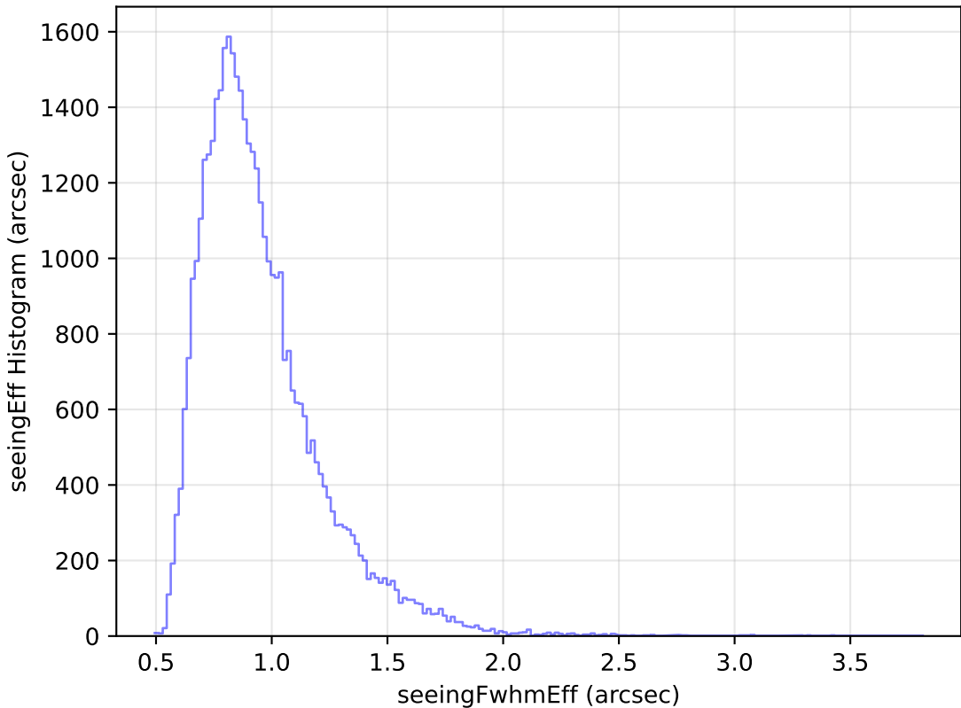
noroll_mjdp270_v3.4_10yrs Yr 1 z band: seeingEff Histogram
