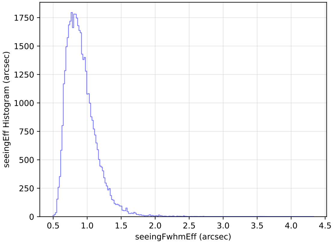
noroll_mjdp270_v3.4_10yrs Yr 1 y band: seeingEff Histogram
