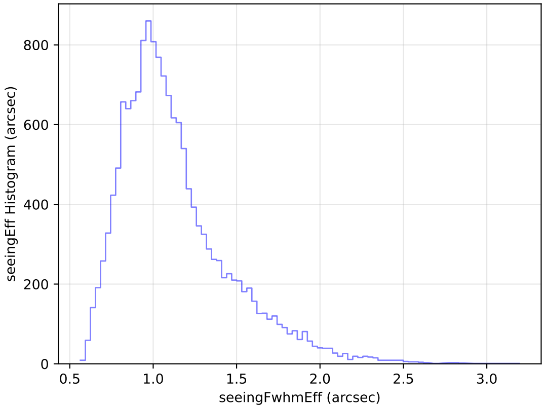
noroll_mjdp270_v3.4_10yrs Yr 1 u band: seeingEff Histogram
