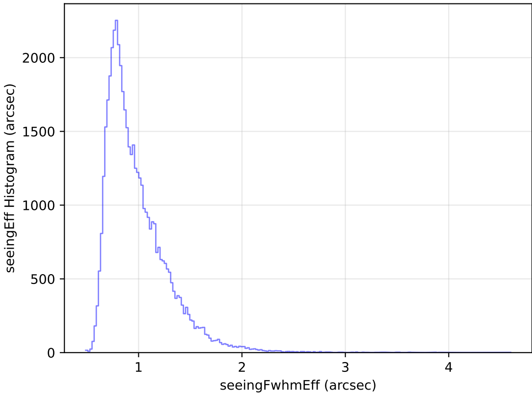
noroll_mjdp270_v3.4_10yrs Yr 1 r band: seeingEff Histogram
