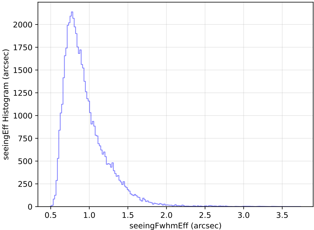
noroll_mjdp270_v3.4_10yrs Yr 1 i band: seeingEff Histogram
