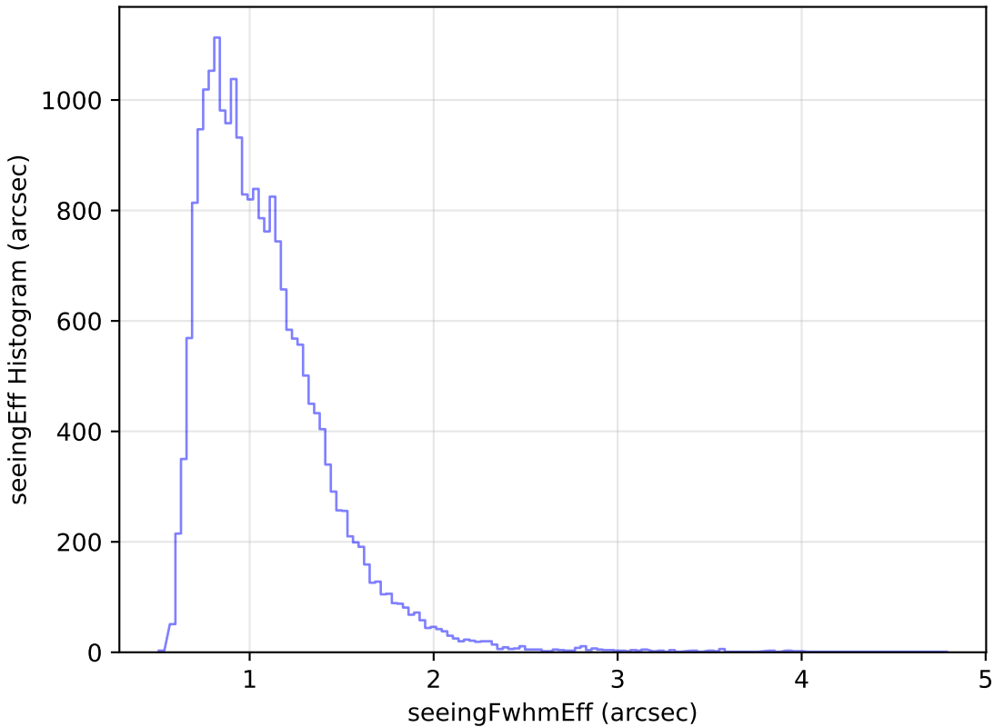
noroll_mjdp270_v3.4_10yrs Yr 1 g band: seeingEff Histogram
